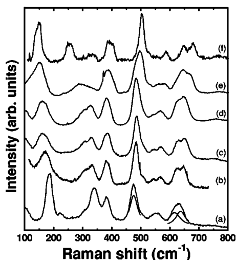
FIG. 3. Room temperature Raman spectra of \text{Hf}_x\text{Zr}_{1-x}\text{O}_2 nanoparticles after sintering at 1200 °C in air for 1 h, taken with at \lambda = 514.5 nm: (a) \text{ZrO}_2 , (b) \text{Hf}_{0.12}\text{Zr}_{0.88}\text{O}_2 , (c) \text{Hf}_{0.45}\text{Zr}_{0.55}\text{O}_2 , (d) \text{Hf}_{0.46}\text{Zr}_{0.54}\text{O}_2 , (e) \text{Hf}_{0.75}\text{Zr}_{0.25}\text{O}_2 , and (f) \text{HfO}_2 . The Lorentzian fits of the M12 (475 \text{cm}^{-1} ), M16 (616 \text{cm}^{-1} ), and M17 (637 \text{cm}^{-1} ) peaks that are used for composition analysis are shown only in (a).
