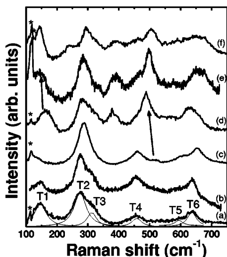
FIG. 1. Room temperature Raman spectra of \text{Hf}_x\text{Zr}_{1-x}\text{O}_2 nanoparticles after heating at 600 °C in air for 1 h, taken with at \lambda = 514.5 nm: (a) \text{ZrO}_2 , (b) \text{Hf}_{0.12}\text{Zr}_{0.88}\text{O}_2 , (c) \text{Hf}_{0.45}\text{Zr}_{0.55}\text{O}_2 , (d) \text{Hf}_{0.46}\text{Zr}_{0.54}\text{O}_2 , (e) \text{Hf}_{0.75}\text{Zr}_{0.25}\text{O}_2 , and (f) \text{HfO}_2 . The Lorentzian fits of the peaks are shown only in (a). Peaks labeled T1–T6 are the six tetragonal phase first order Raman modes. The two arrows point from monoclinic phase peaks in spectra of lower x to the same peaks at higher x . Plasma lines from the laser are denoted by an asterisk.
